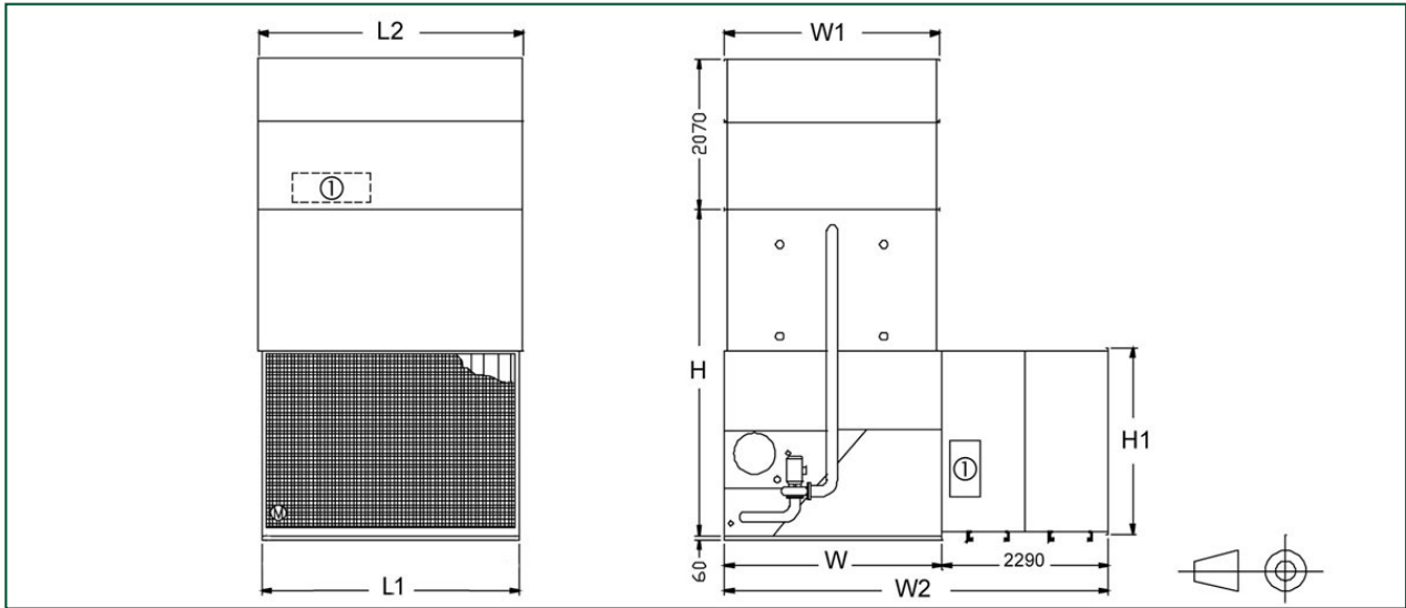
1. Access door; L = Unit Length; W = Unit Width; H = Unit Height (see Engineering data).
