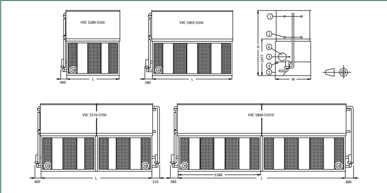
1. Refrigerant in ND100; 2. Refrigerant out ND100; Make up ND50; 4. Overflow ND80; 5. Drain ND50; 6. Access.
